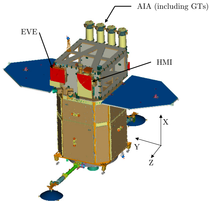
Figure 1: SDO spacecraft with instruments labeled.
