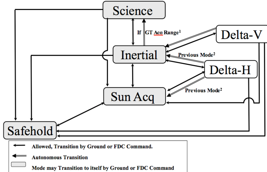
Figure 6: ACS Control Mode Transition Diagram
