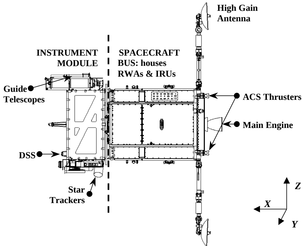
Figure 1: Solar Dynamics Observatory side view
