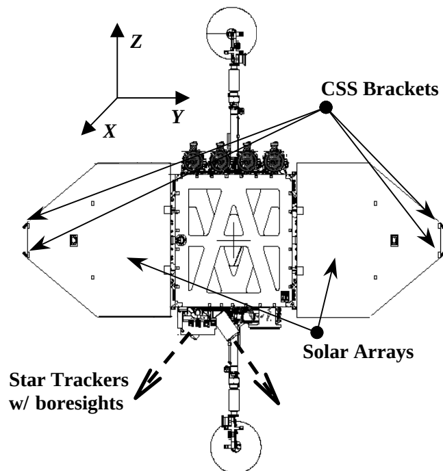
Figure 2: SDO Solar Array View
