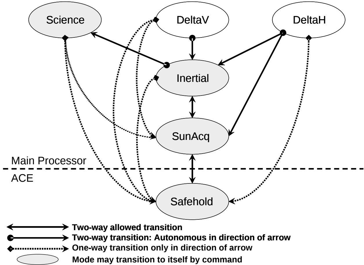
Figure 3: Allowed mode transitions for SDO ACS software
